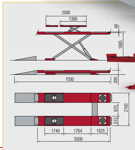
RAV 650.2.55SI - 5000 kg Assetto/Alignment
